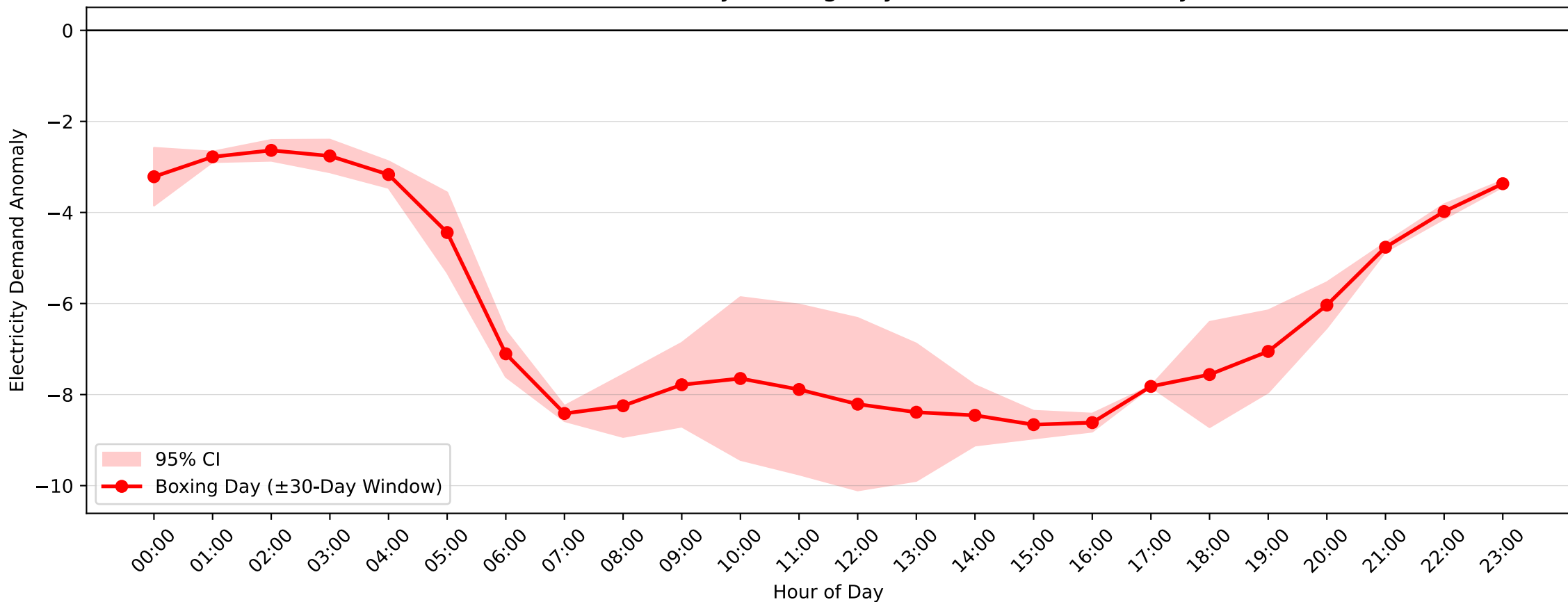
Dulwich Hill Demand Anomaly: Boxing Day (2006–2007, \pm 30 -Day Window)
