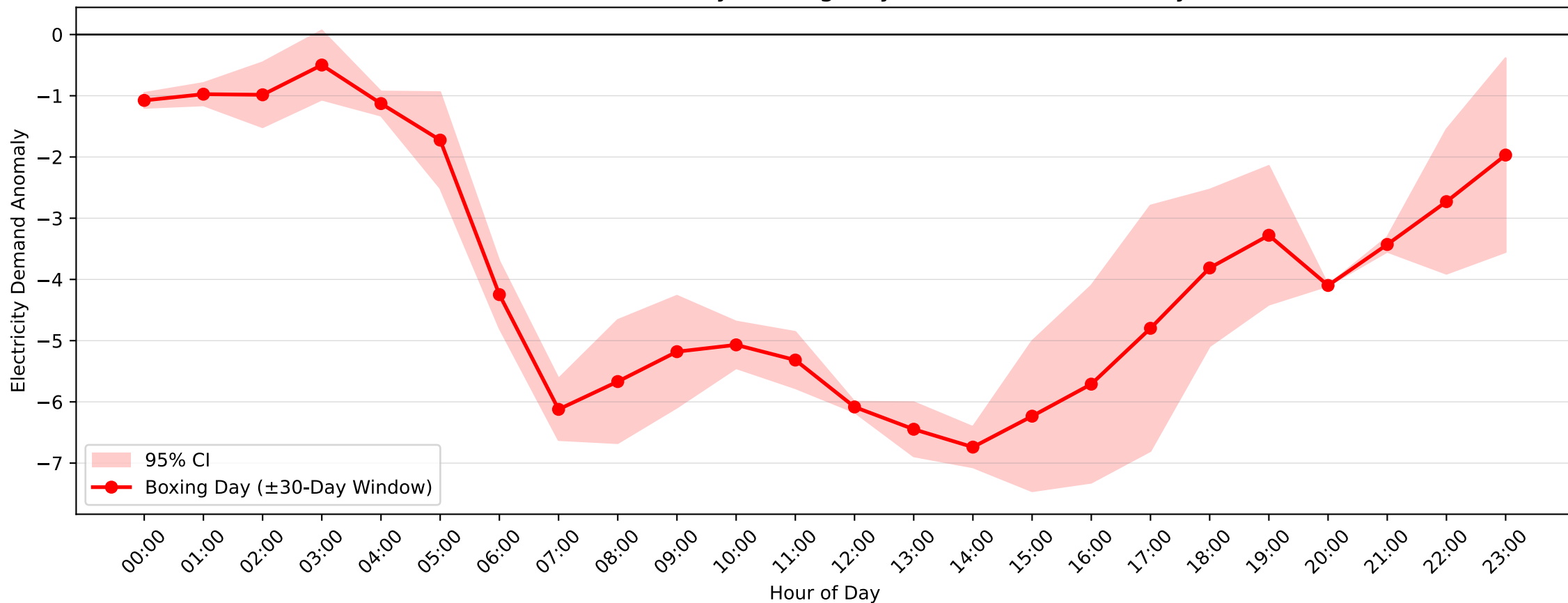
Dulwich Hill Demand Anomaly: Boxing Day (2009–2010, \pm 30 -Day Window)
