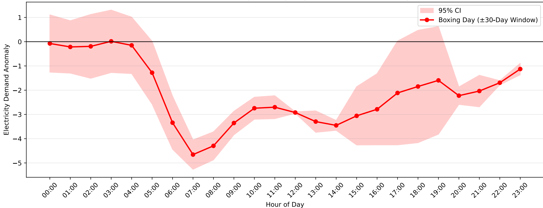
Dulwich Hill Demand Anomaly: Boxing Day (2010-2011, \pm 30 -Day Window)
