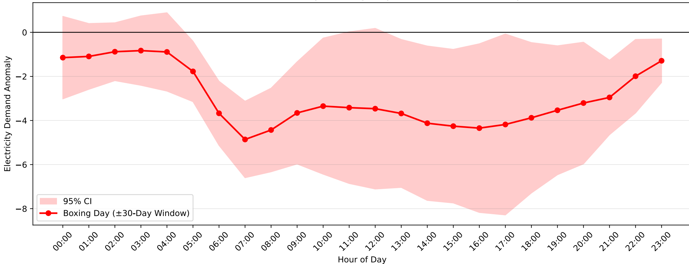
Dulwich Hill Demand Anomaly: Boxing Day (2011-2012, \pm 30 -Day Window)
