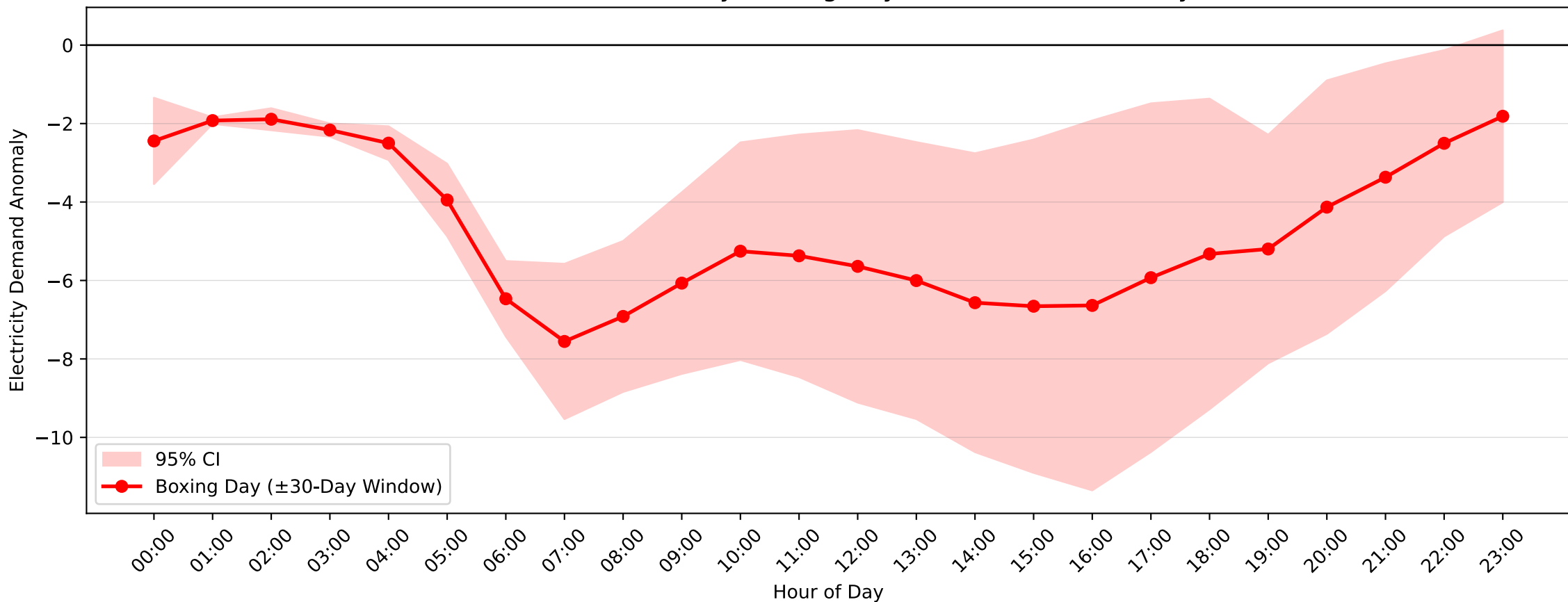
Dulwich Hill Demand Anomaly: Boxing Day (2007-2008, \pm 30 -Day Window)
