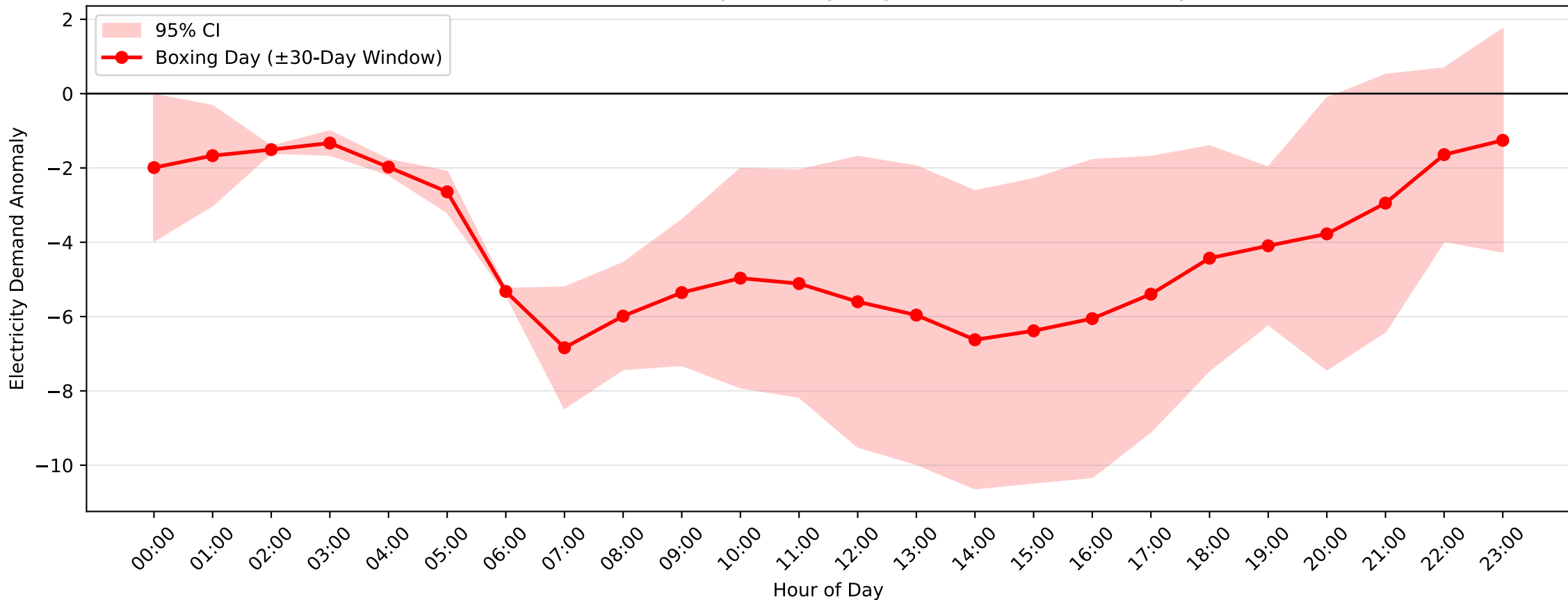
Dulwich Hill Demand Anomaly: Boxing Day (2008-2009, \pm 30 -Day Window)
