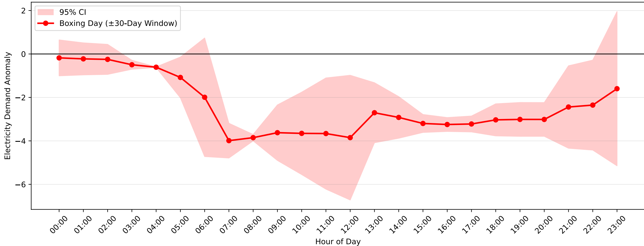
Dulwich Hill Demand Anomaly: Boxing Day (2014–2015, \pm 30 -Day Window)
