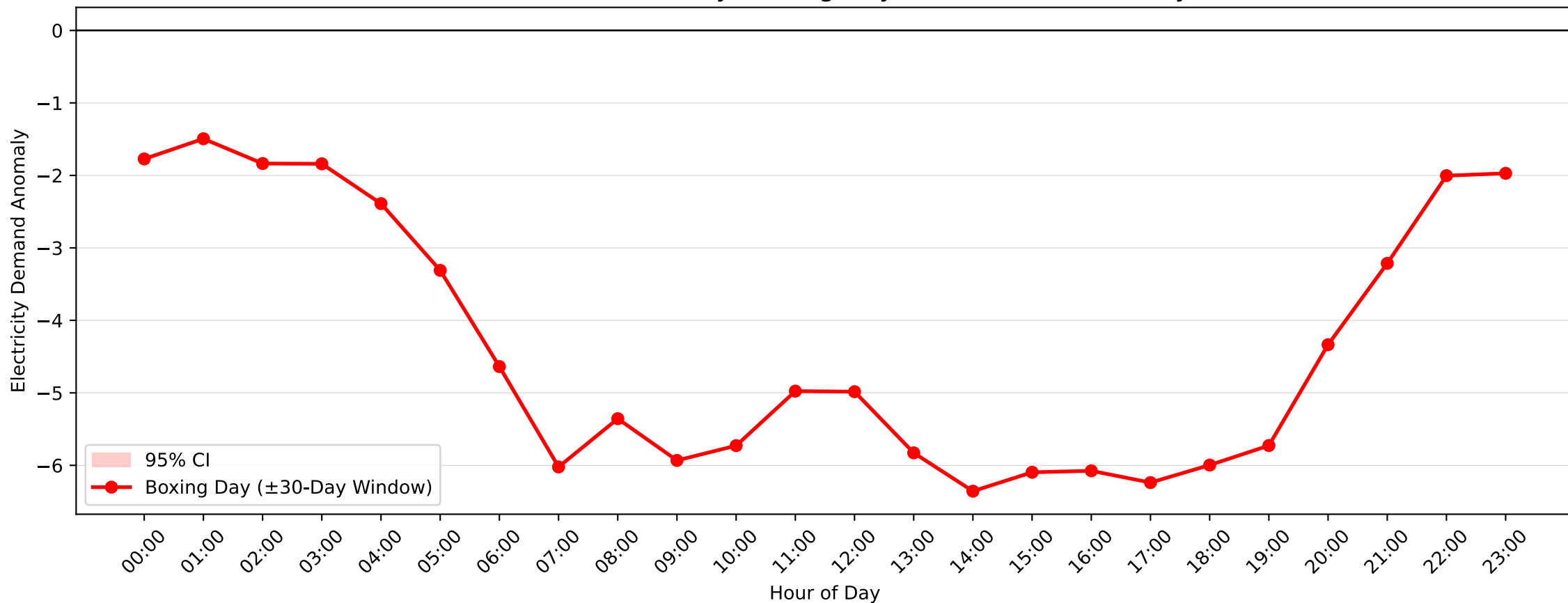
Dulwich Hill Demand Anomaly: Boxing Day (2004–2005, \pm 30 -Day Window)
