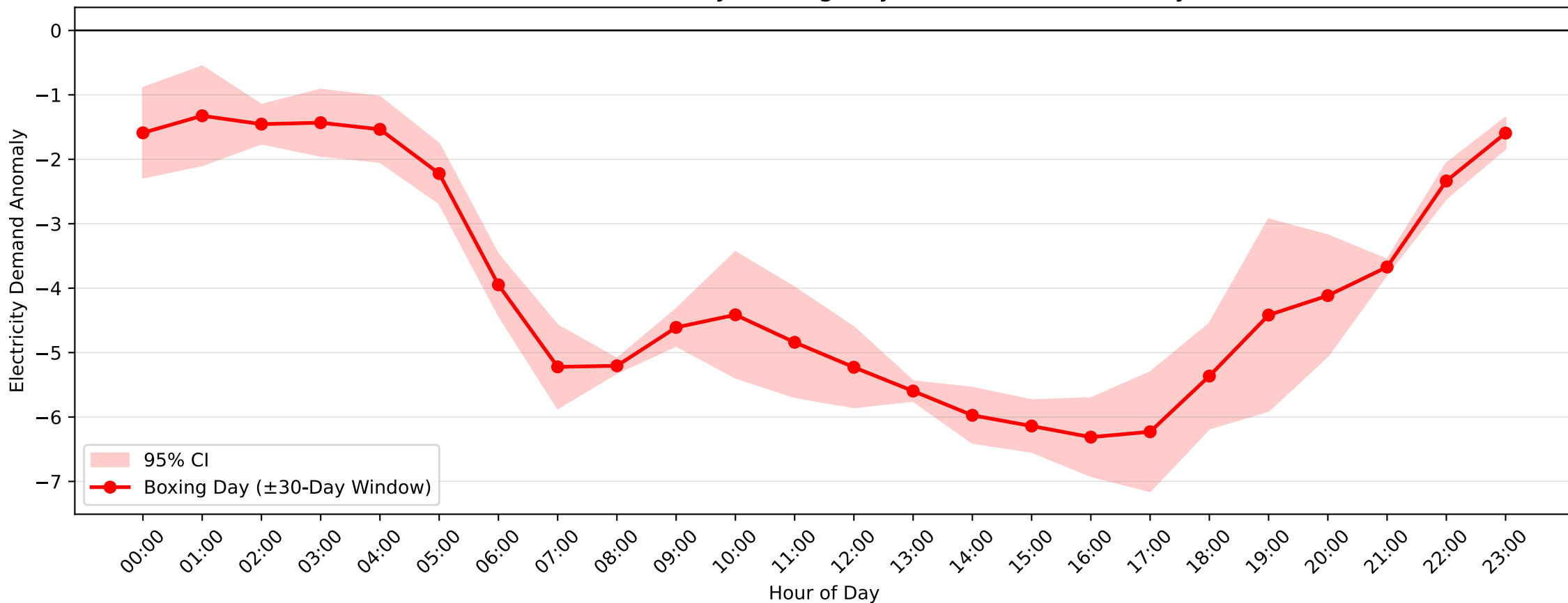
Dulwich Hill Demand Anomaly: Boxing Day (2012–2013, \pm 30 -Day Window)
