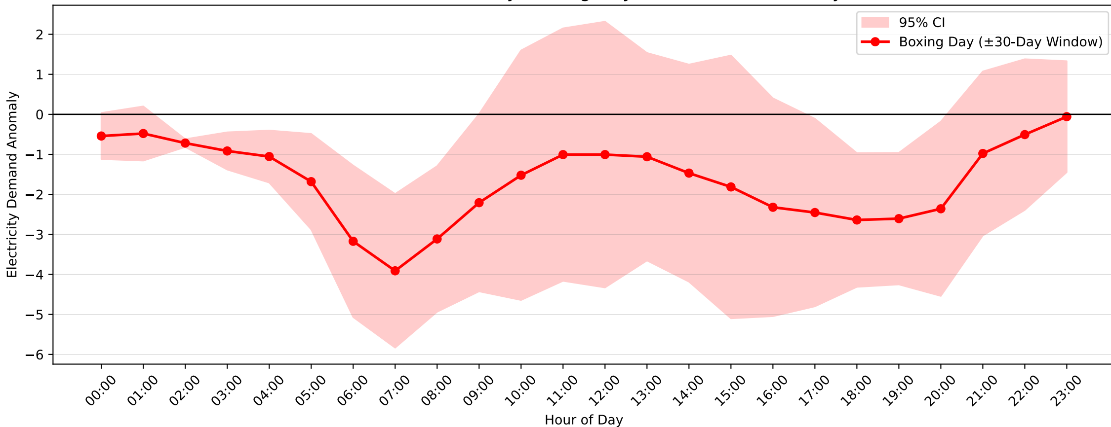
Dulwich Hill Demand Anomaly: Boxing Day (2015–2016, \pm 30 -Day Window)
